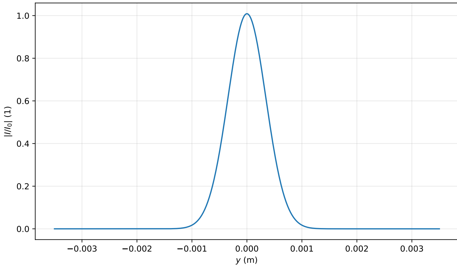
Intensity profile I(x=0, y, z=0.159)/I_0 , P_{in}=0.6P_{cr} , artificial time
